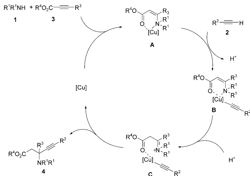
Scheme 3. Tentative mechanism for the copper-catalyzed amine-alkyne-alkyne addition.
