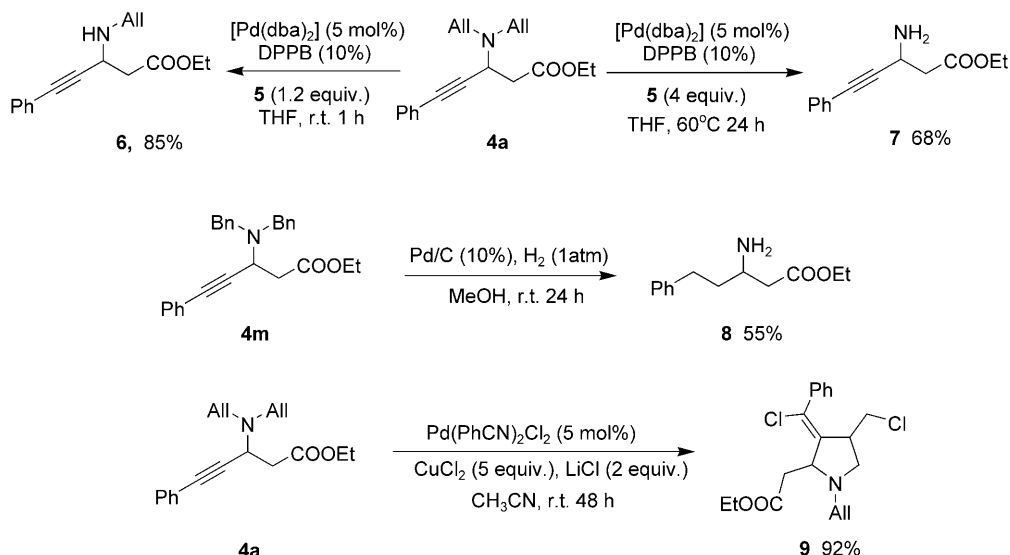
Scheme 2. Selective transformations of \gamma,\delta -alkynyl- \beta -amino acid derivatives.
